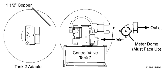
Figure 2 9500 Equipment Configuration
