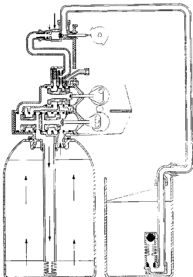
2 Backwash Position
